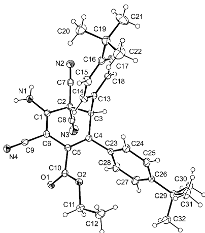
Fig. 2 Molecular structure of intermediate F in the crystal.
